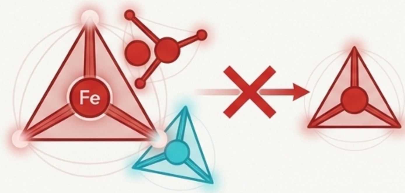
Reaction Blocked
