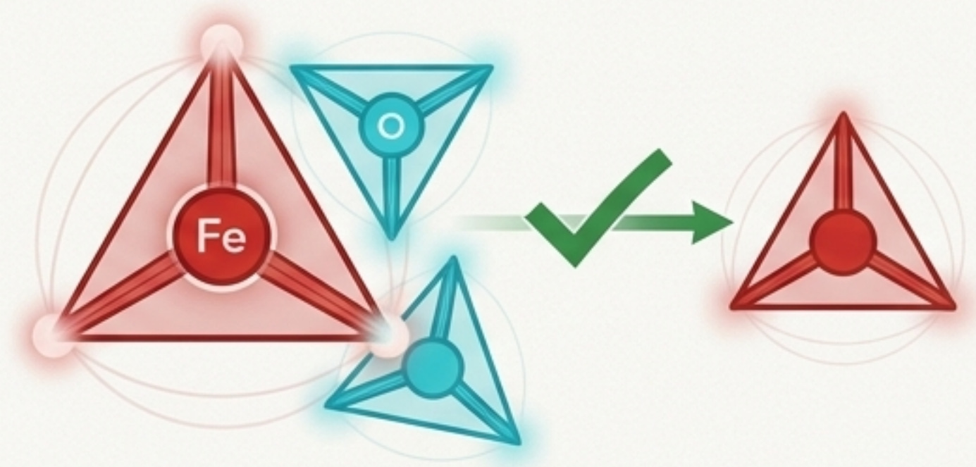
Reaction Proceeds
